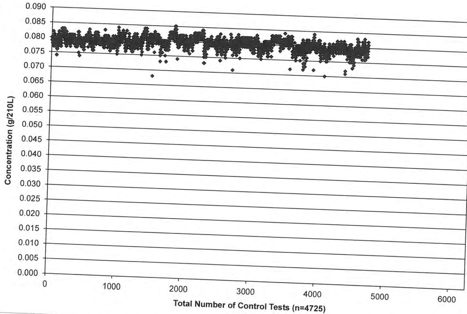
November 2018 Control Tests Chart (All Control Tests) Includes Control Tests Flagged Control Outside Tolerance (n=23), Interferent Detect (n=8) and RFI Detect (n=3)
