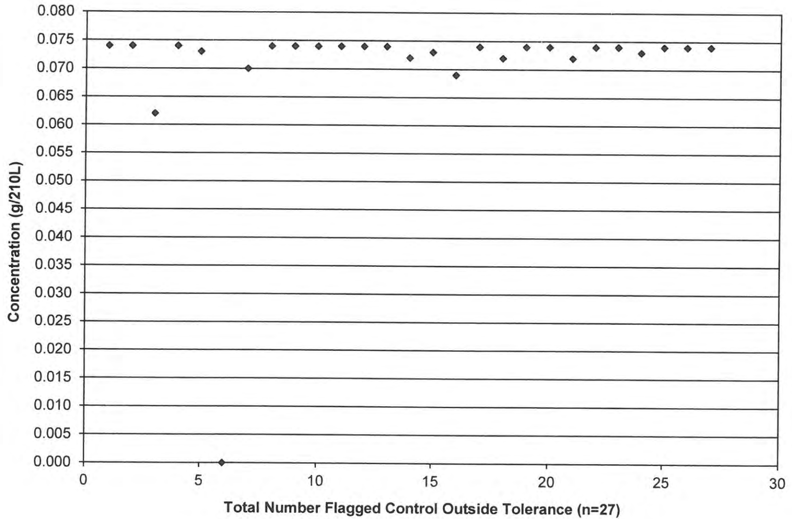
July 2018 Control Tests Flagged Control Outside Tolerance
